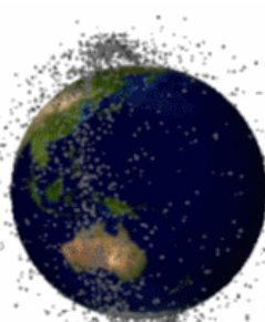
Predicted lifespan of FY-1C debris on orbit 7
