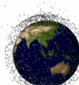
Predicted lifespan of FY-1C debris on orbit 7
