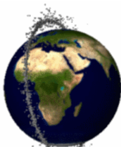
Debris cloud after 10 days
